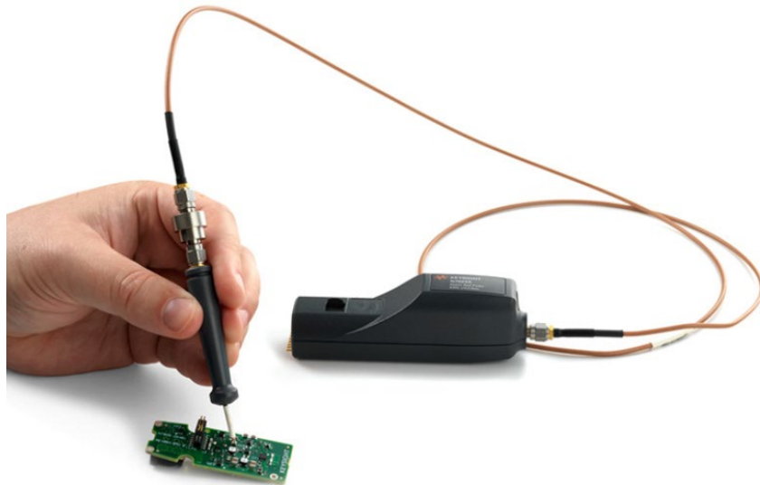
Figure 16. Notice how the rotating adapter isolates the browser from the natural torque or twist of the probe main cable.
