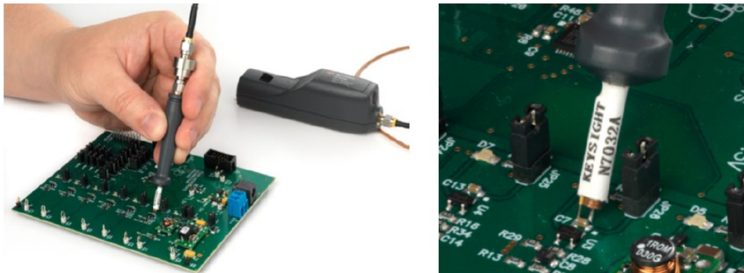
Figure 13. The N7032A 4 GHz power rail probe browser and closer view when probing a small capacitor package on the power distribution network
