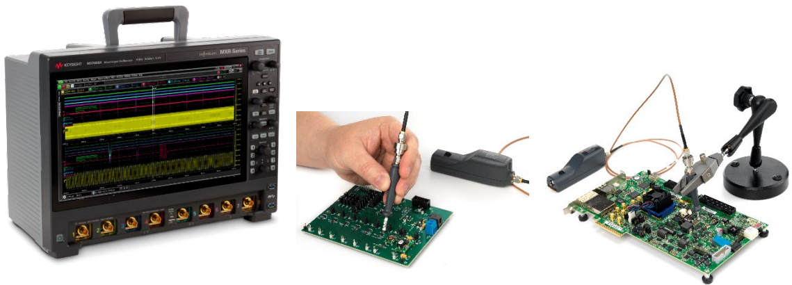
Figure 7. The N7024A Power Rail probe with Infiniium MXR-Series Oscilloscope to make a power integrity measurement
