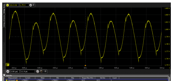
Figure 1. Using the N7020A power rail probe, with 2 GHz bandwidth and 50 k \Omega DC resistive loading, to see the AC and DC components of a DC power rail.
