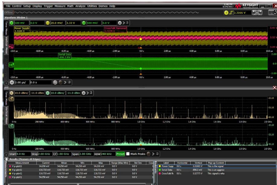
Figure 24. Output from the D9010POWA PI application showing a reduction in the noise on the 3.3 V supply after the effects of the switching loads were removed.
