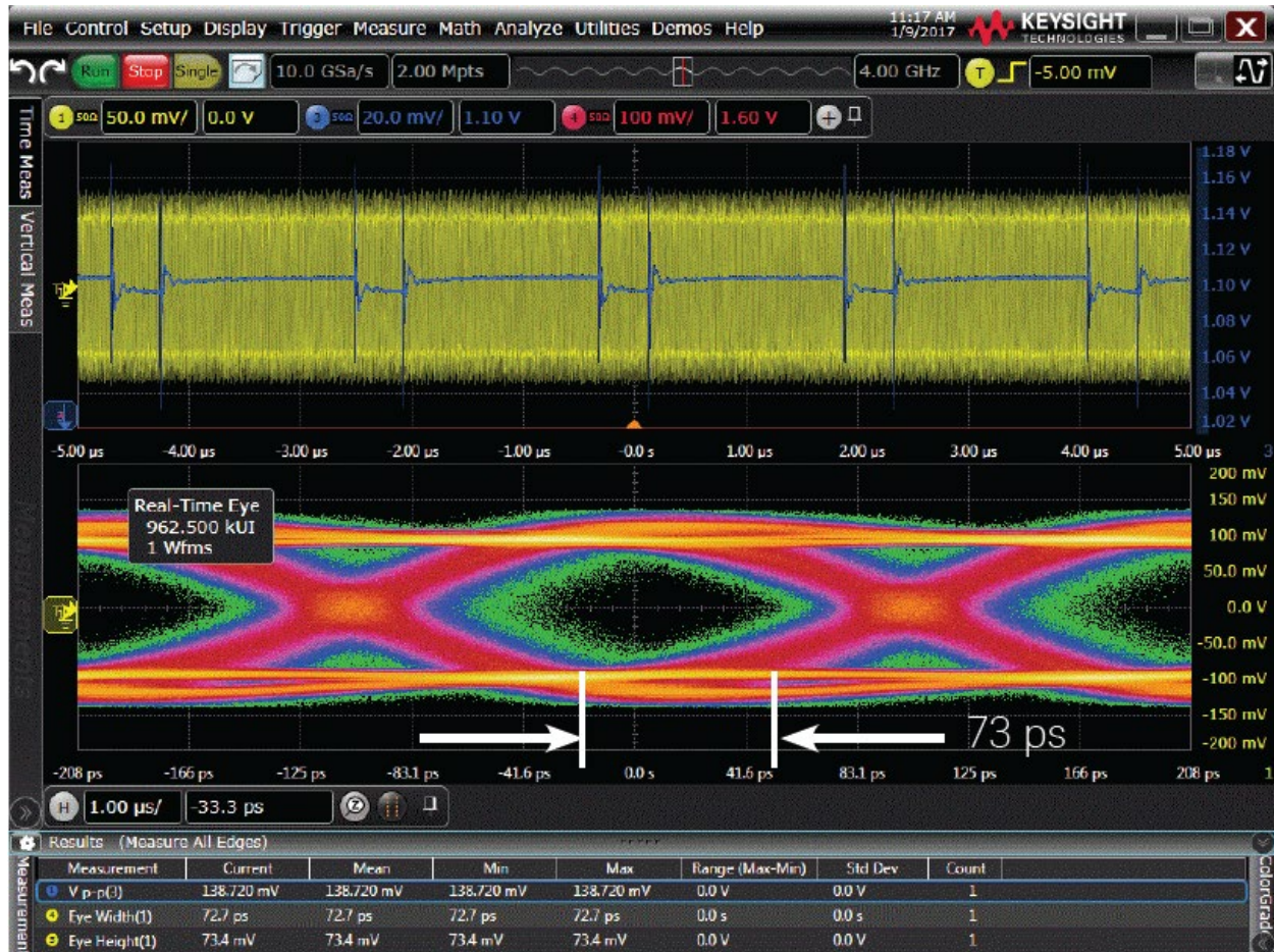
Figure 18. Eye diagram of FPGA serial data affected by DC supply noise.
