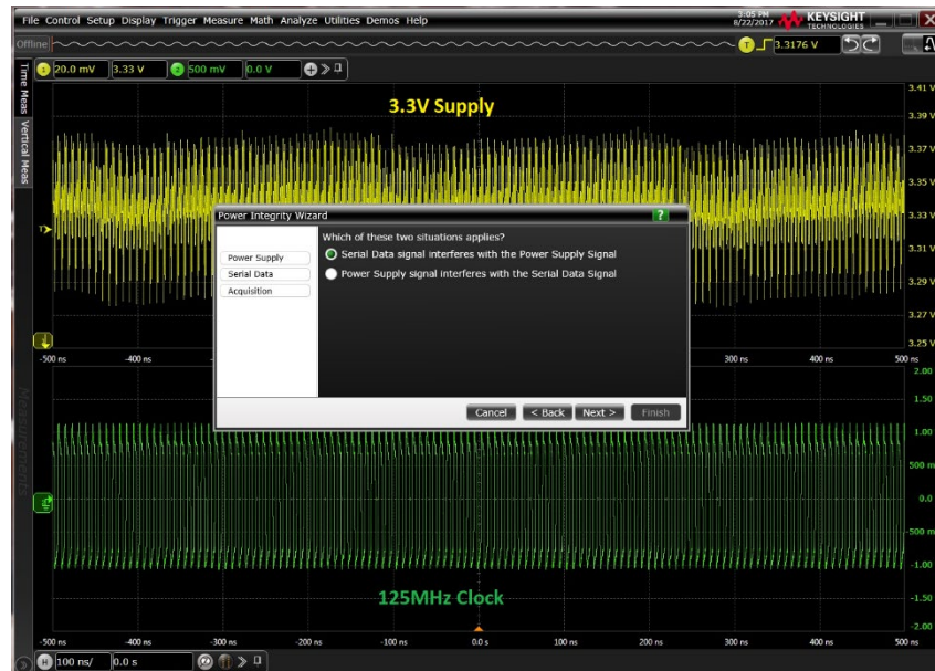
Figure 23. The clock of the digital was probed and is being analyzed as the aggressor to the power rail as shown in the PI setup wizard dialogue (next page).
