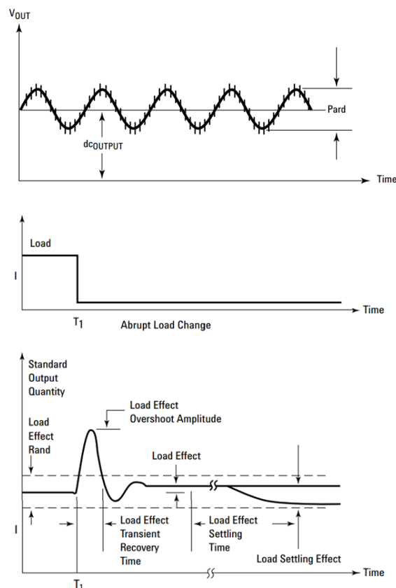
Figure 5. Examples of types of power integrity measurements
