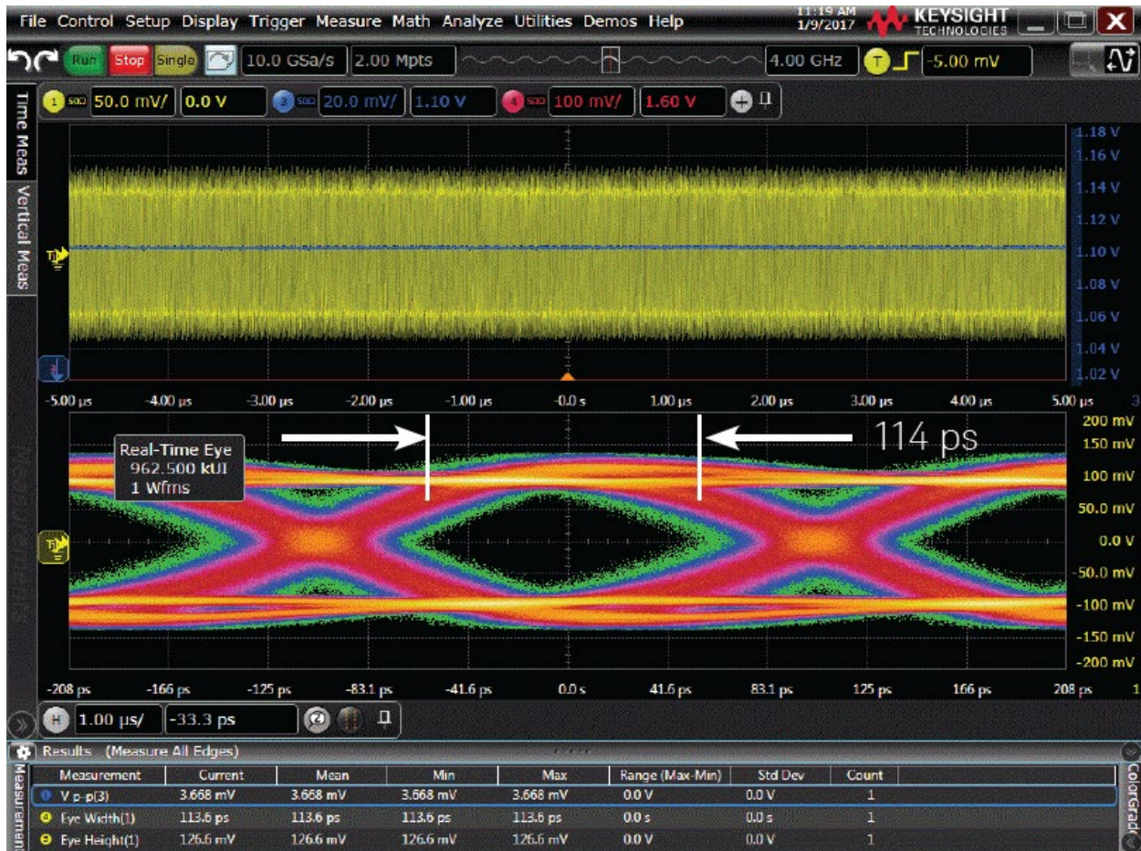
Figure 19. Eye diagram of FPGA serial data after the DC supply was cleaned-up. Notice the increased width of the eye.
