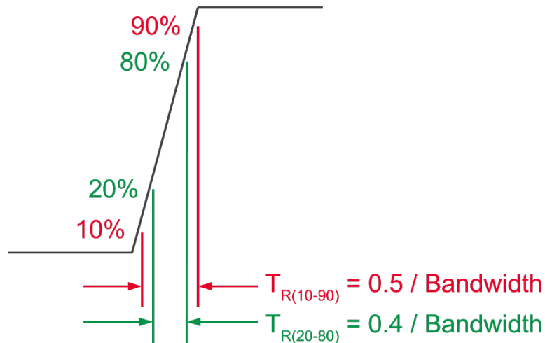
Figure 6. Probe rise time specifications maximally flat response probes and the relationship between rise time and bandwidth at different thresholds.
