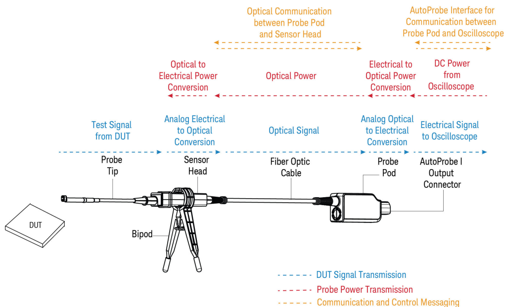
Figure 4 Working of the PS0004A/6A/8A Probes
