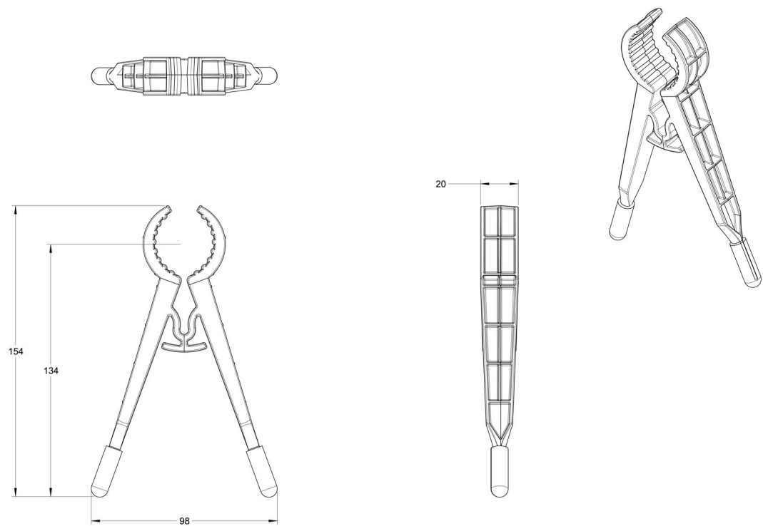
Figure 19 Bipod Dimensions
