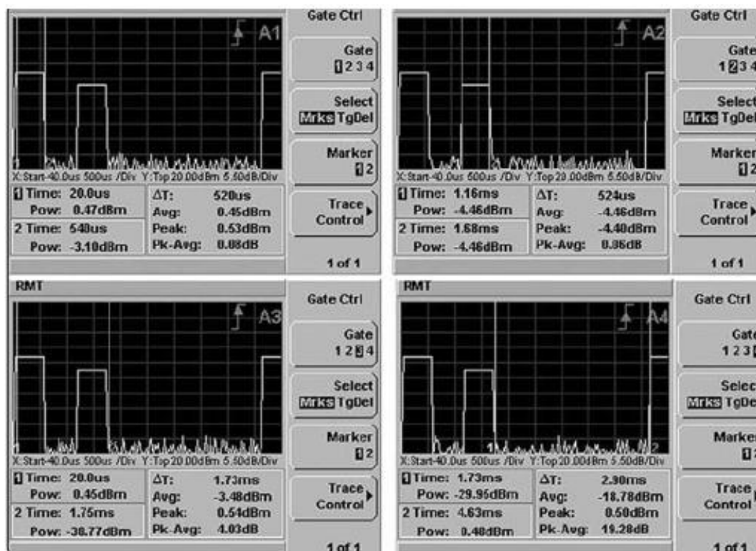
Figure 9. Measurement flexibility with four independent time gates
