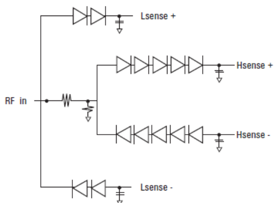
Figure 5. Simplified block diagram of the two-path-diode-stack topology.
