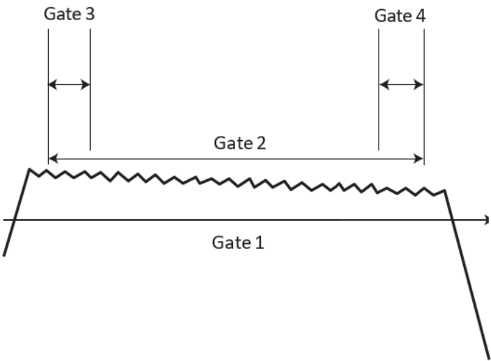
Figure 15. On this GSM pulse, powerful data configuration routines during four gate times, provide the feeds for the display.
