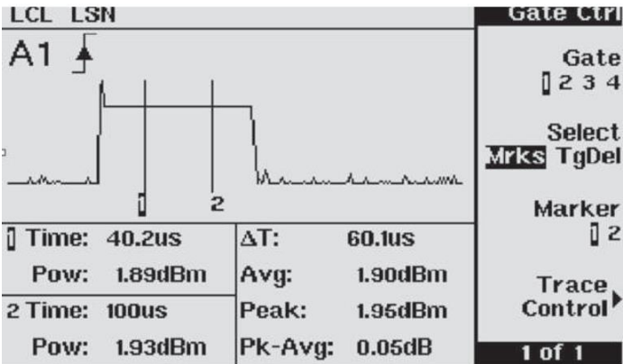
Figure 16. This graphical display permits marker-selected power measurements, plus computations between the marker-identified data.
