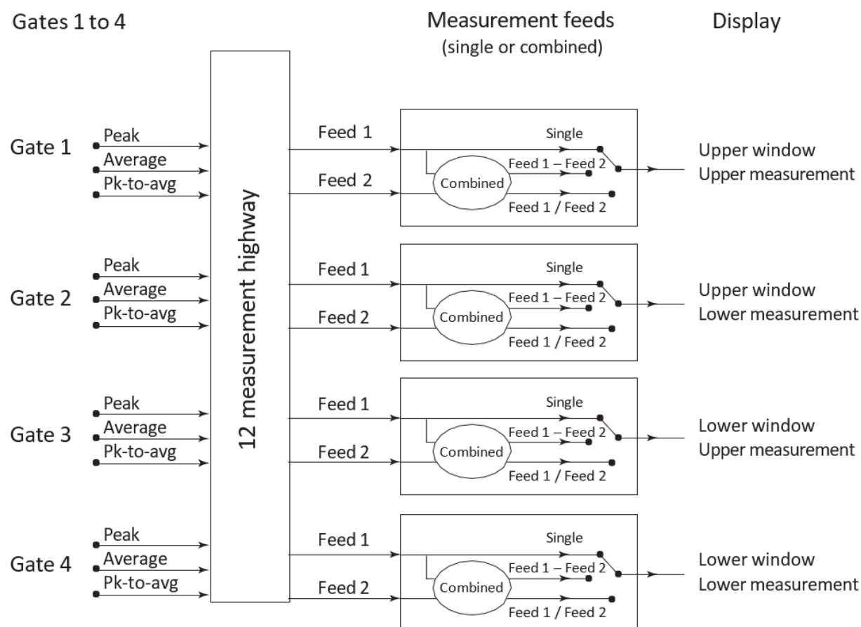
Figure 20. User-configured data manipulations: a major feature of the EPM-P Series power meters.
