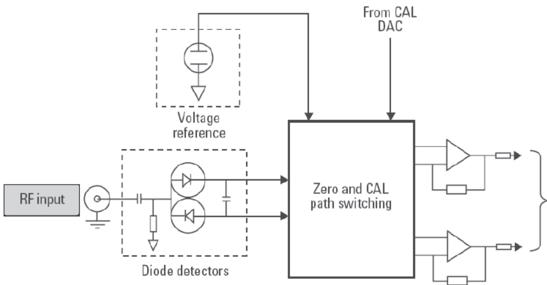
Figure 6. Internal zero and cal block diagram
